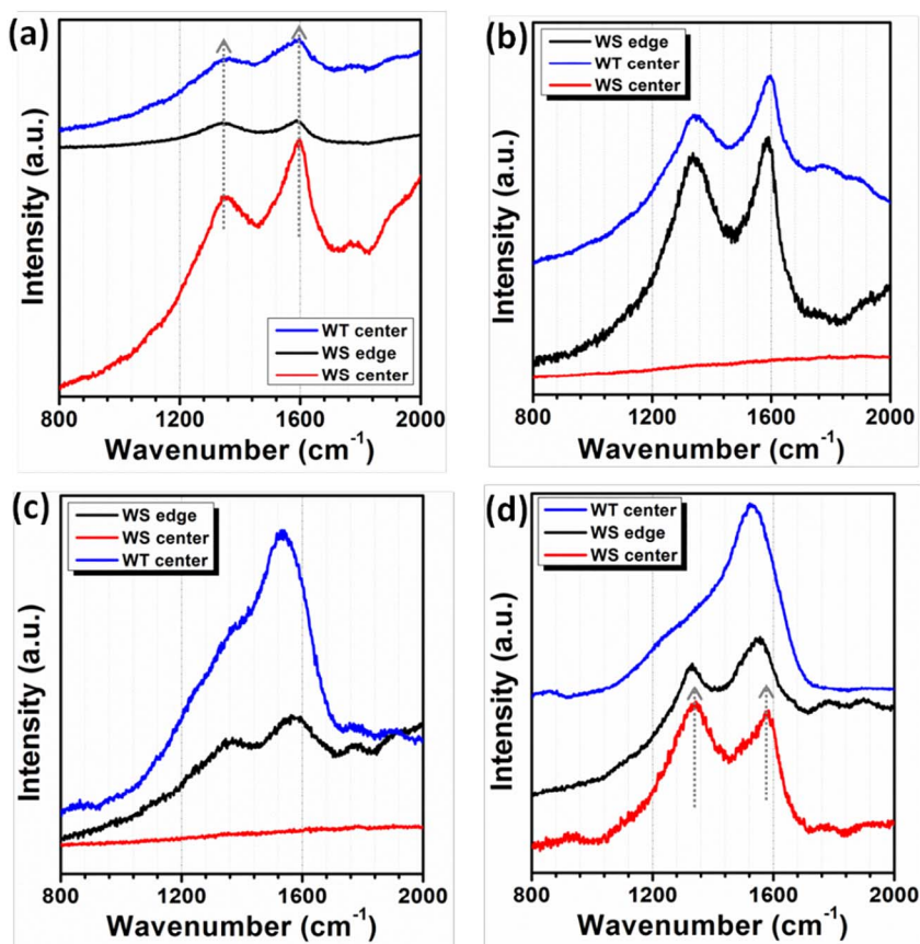
Fig. 6. Micro-Raman spectra of WT center, WS center and WS edge on uncoated \text{Al}_2\text{O}_3 surface in (a) dry nitrogen, (b) dry oxygen, (c) dry argon atmospheres and (d) on a-C:H coated \text{Al}_2\text{O}_3 surface in dry nitrogen. (WT: wear track, WS: wear scar).
