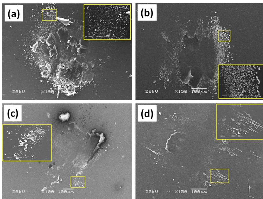
Fig. 7. SEM pictures of wear scar areas on uncoated \text{Al}_2\text{O}_3 balls sliding against a-C:H films in (a) \text{N}_2 , (b) \text{O}_2 , (c) Ar and (d) on coated \text{Al}_2\text{O}_3 surface in dry \text{N}_2 atmospheres. Insets show the corresponding enlarged SEM pictures of framed areas.
